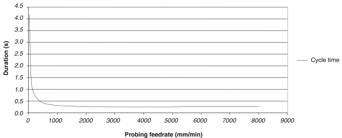
Figure 2: Single touch cycle time
