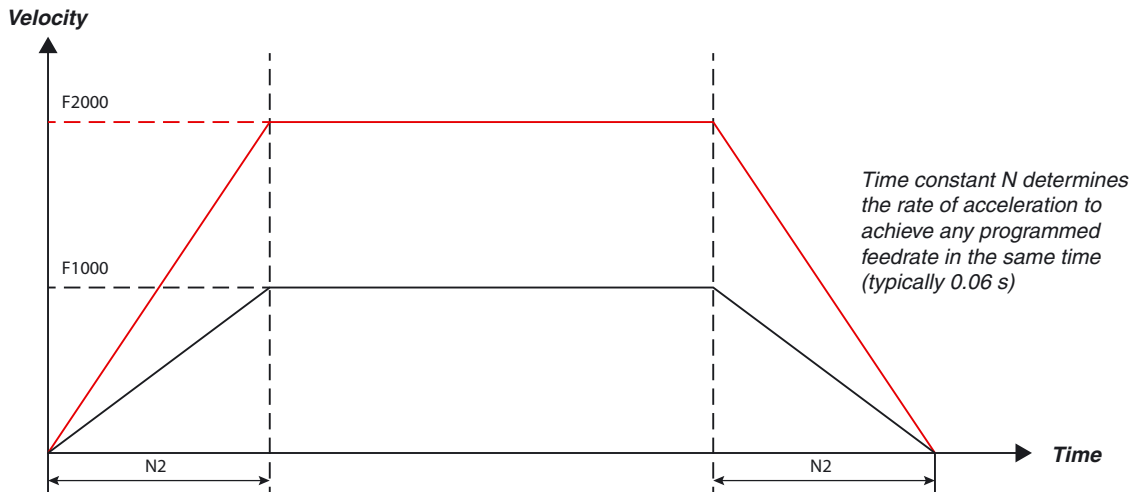
Figure 1: Machine accelerates over a set period of time, making the rate of acceleration dependent on the feedrate required
