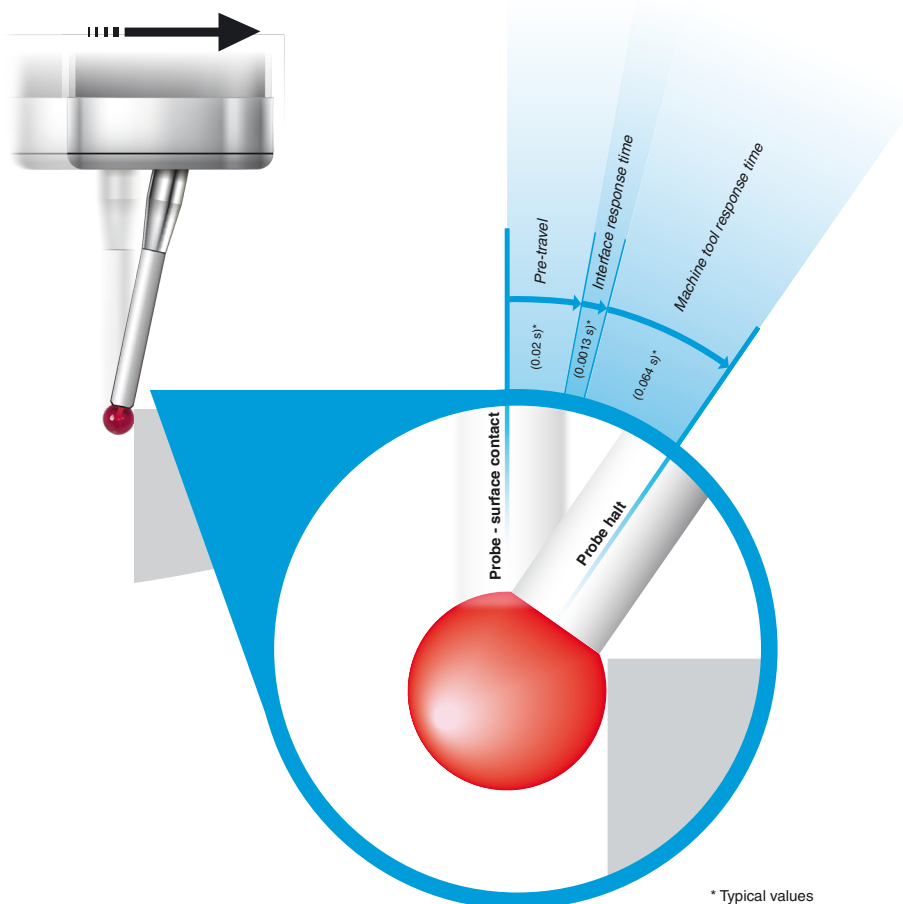
Figure 3: Probe trigger sequence and signal transmission
